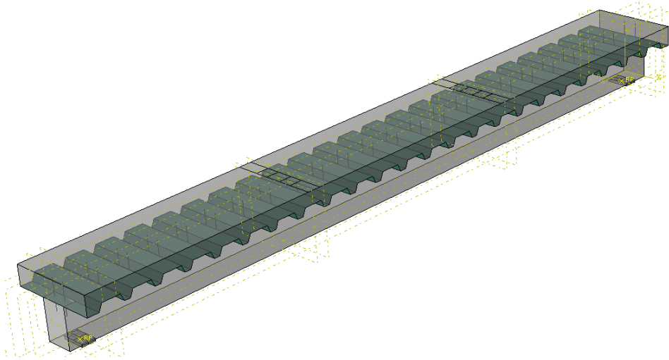
Fig. 2. Steel sheeting as the skin of the concrete slab
