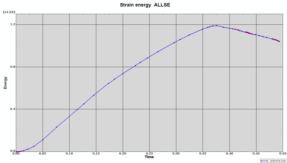
Fig. 10. The strain energy curve
