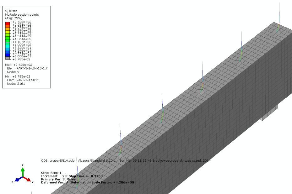
Fig. 7. The stresses of the shear connectors
