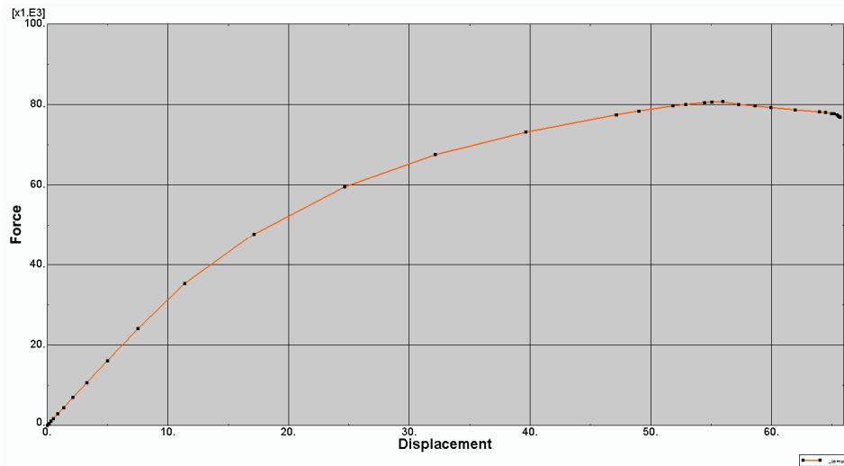
Fig. 9. The static equilibrium path force - displacement for the thinner slab
