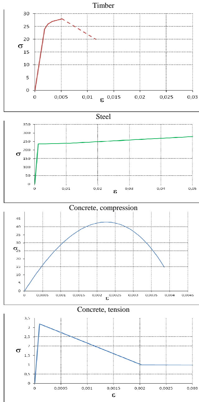
Fig. 5. The laws of physics for each material
