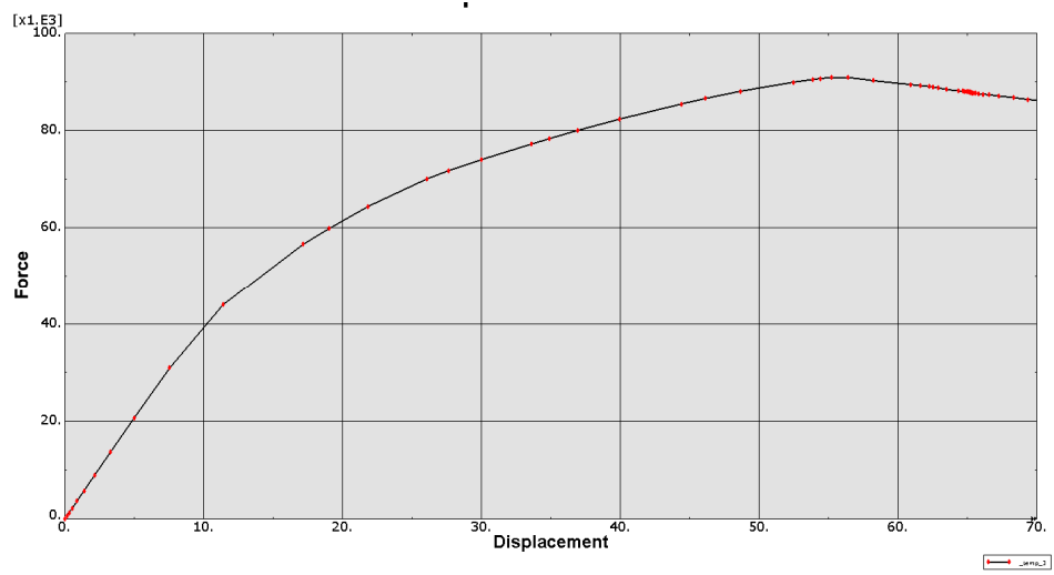
Fig. 6. The static equilibrium path force - displacement
