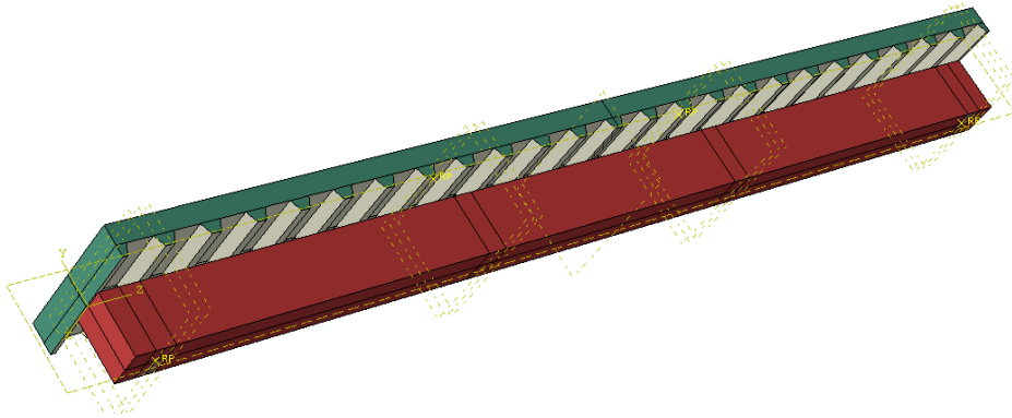
Fig. 1. A 3D model of the composite timber and concrete beam
