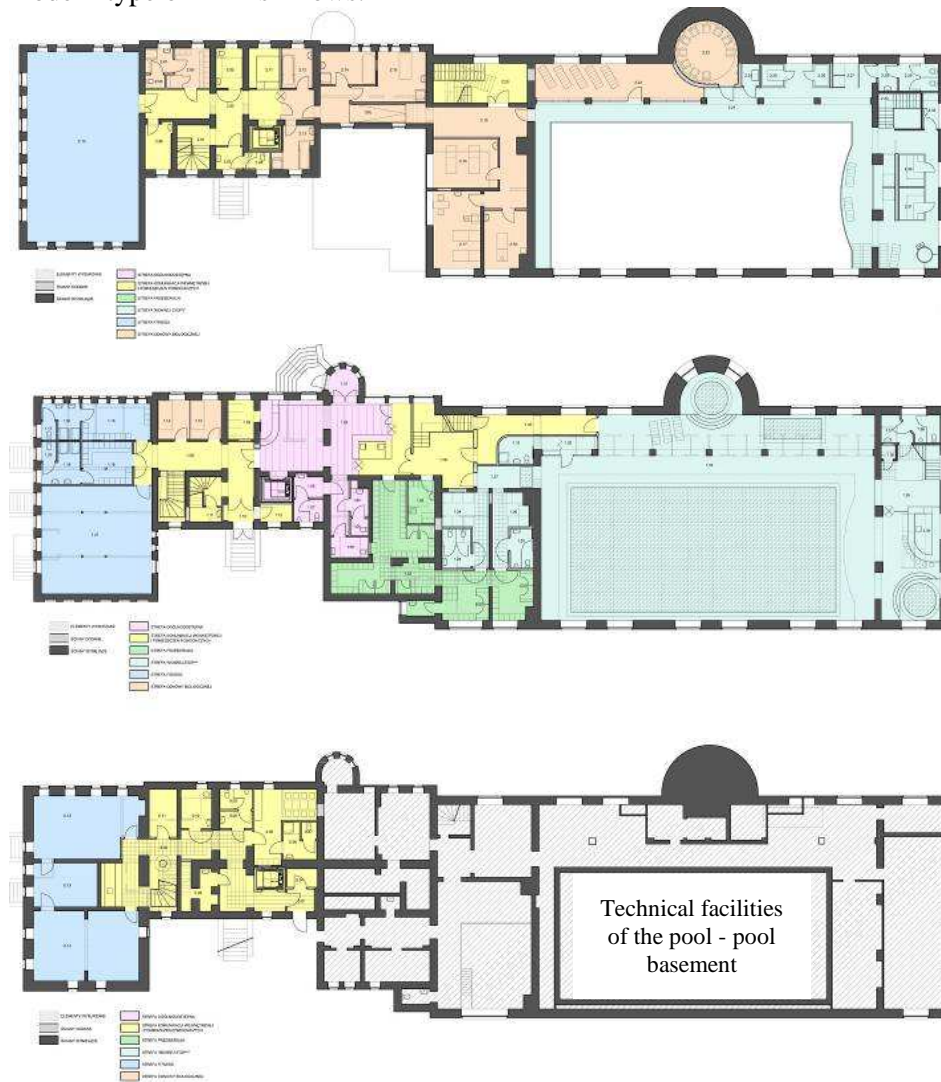
Fig. 1. Plan of the basement, ground and first floors of the building (bottom to top) - the original concept illustrating the distribution of planned functional zones in the facility (based on the conceptual design - from the author's archive)
