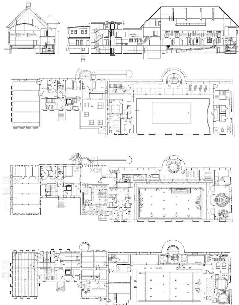
Fig. 3. Plan of the basement, ground and first floors of the building, and cross-sections - version put into implementation ( based on remodelling construction project - from the author's archive )
