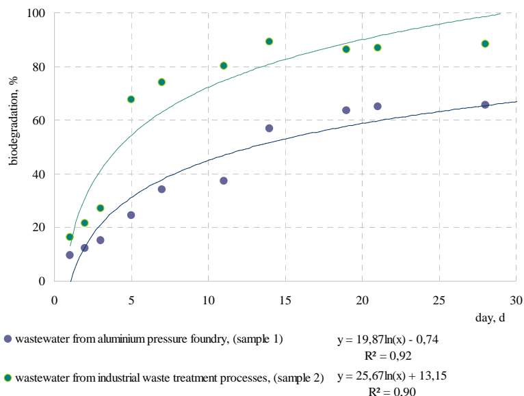
Fig. 1. Substrates degradation curves during Zahn-Wellens test (samples 1 and 2)
