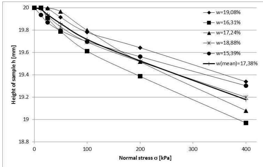
Fig. 2. Diagram of original compressibility of the natural undisturbed samples
