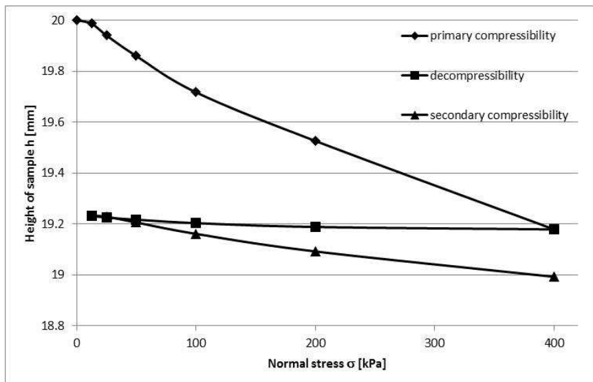
Fig. 3. Diagram of primary compressibility, decompressibility and secondary compressibility of the natural undisturbed samples (mean values)
