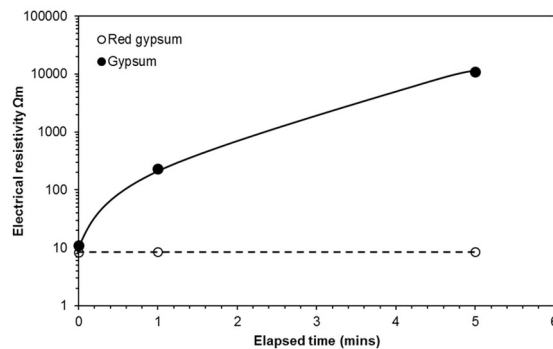
Fig. 1 Evolution of electrical resistivity with elapsed time
