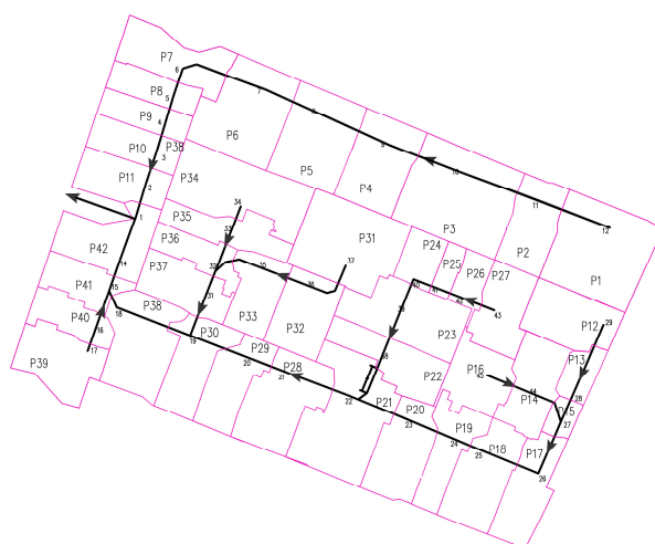
Fig. 2. Diagram of the V catchment - modeled detailed network structure
