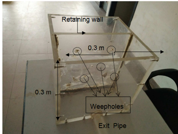
Fig. 6. Fabricated Tank
