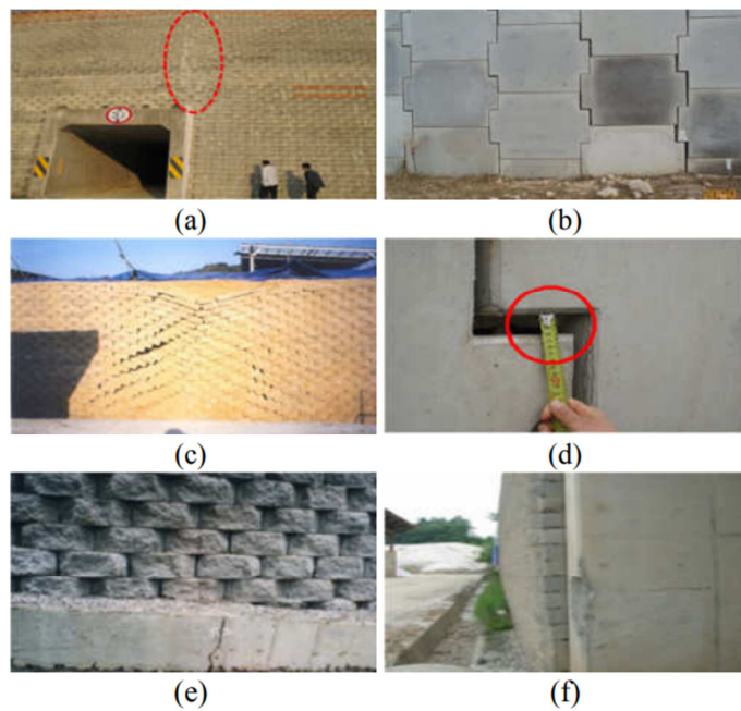
Fig. 3. Excessive settlement and deformation (a) cracking of facing wall, (b) differential settlement of facing wall, (c) settlement of REW, (d) excessive settlement of facing wall, (e) differential settlement of REW, (f) deformation of wall) (Lee and Cho, 2011)
