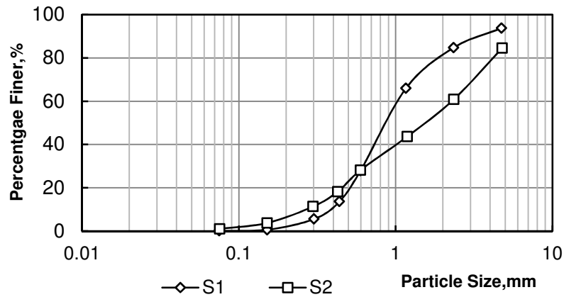
Fig. 4. Soil distribution curve
