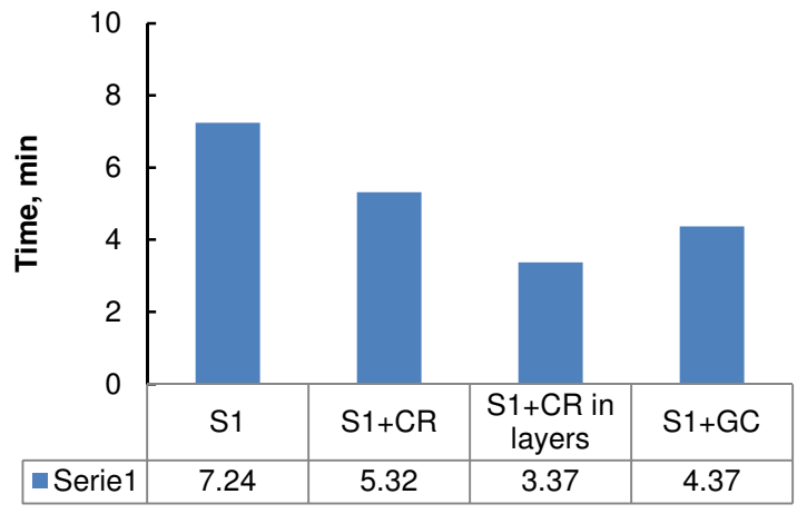
Fig. 10. Comparison of seepage for various materials - S1
