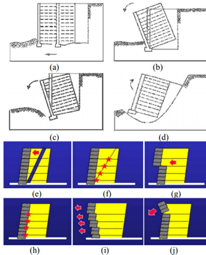
Fig. 1. Failure modes of reinforced earth wall (External failure (a) basal sliding, (b) overturning, (c) bearing capacity failure, (d) overall sliding; internal failure (e) pull-out failure, (f) breakage of reinforcement, (g) internal sliding, (h) breakage of connector, (i) shear failure of facing wall, (j) failure of upper facing block) (Shin et al., 2011)
