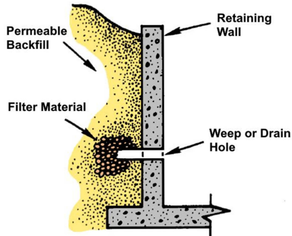
Fig. 2. Location of drains in retaining wall (Froehlich, 2017)
