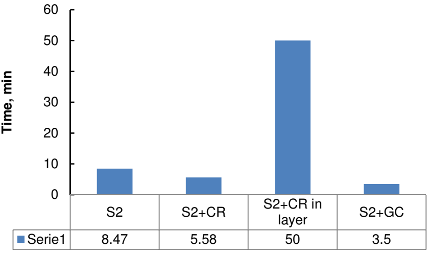
Fig. 11. Comparison of seepage for various materials - S2
