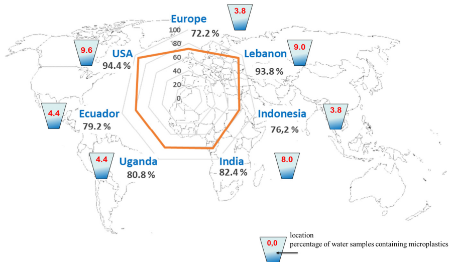
Fig. 2. Measured amount of microplastic particles in tap water (based on [20])
